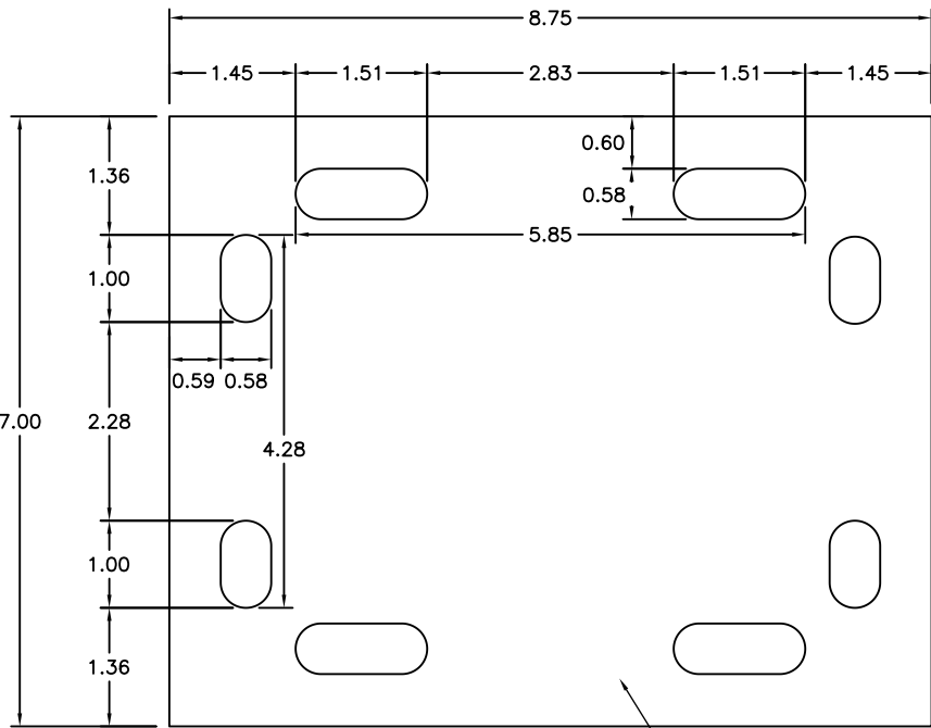
3/8" THICK CROSSOVER PLATE
