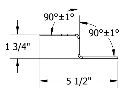
BENT PROFILE
