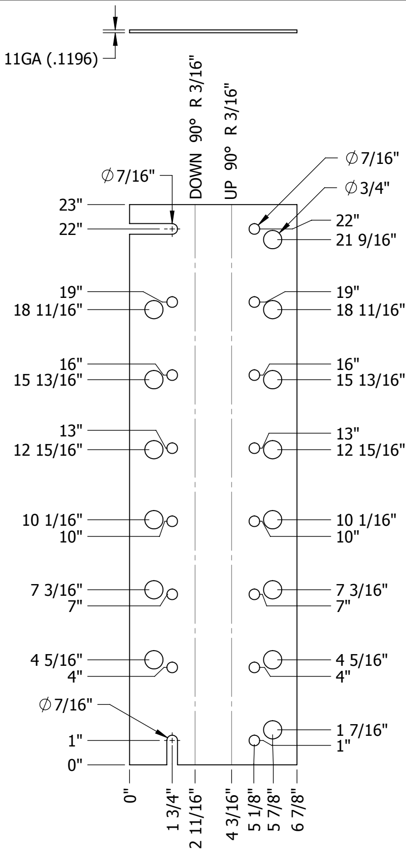
FLAT PATTERN
