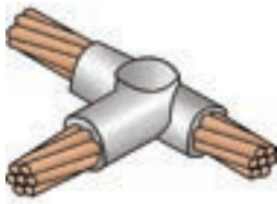
WT 2AS-2AS #2 Solid #2 Solid Tee Connection #45 Shot
