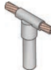
GET-15-2/0A Ground Rod T Over 5/8" Rod, 2/0 wire #90 Shot
