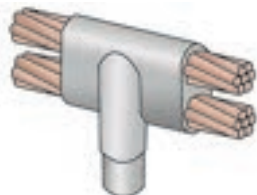
GEP-12-2AS #2 Solid wire to 1/2" Ground Rod Mold #115 Shot
