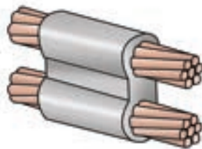
WP-40-2AS #2 Solid Parallel Stack 4/0 Run #150 Shot
