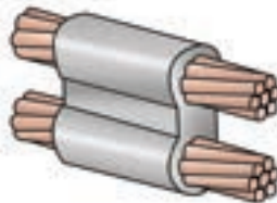
WP-2/0A-2AS #2 Solid 2/0 Stranded Wire Through to Parallel #2 Solid Wire through #90 Shot
