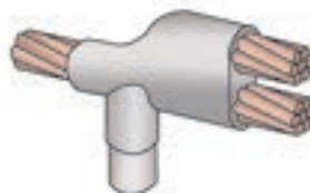
GEY-15-2AS Ground Rod Y-Over 5/8" Rod, (2) #2 Solid #115 Shot
