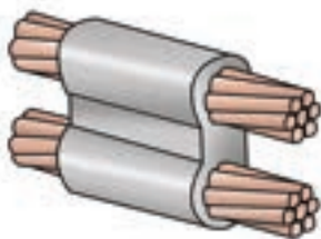
WP-2AS-2AS #2 Solid #2 Solid Parallel Connection #65 Shot
