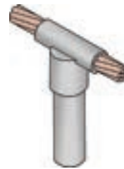
GET-12-2AS #2 Solid 1/2" Ground Rod #65 Shot
