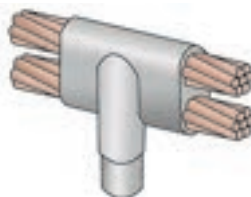
GEP-15-2AS #2 Solid Parallel through over 5/8 Ground Rod #150 Shot
